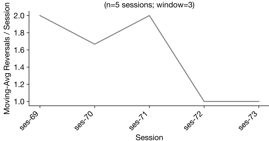
MY_72_R (n=5 sessions; window=3)
